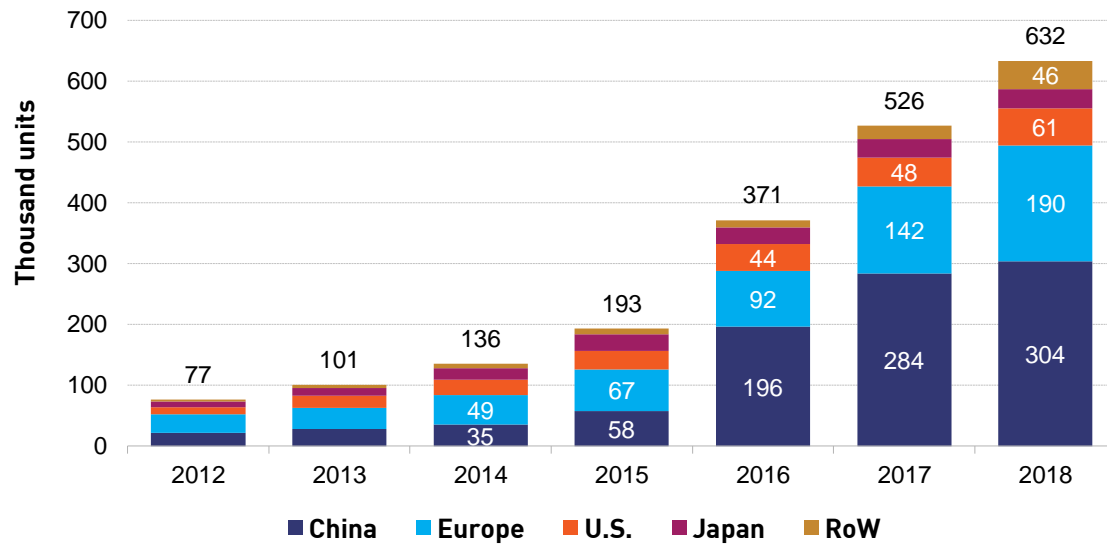
Global cumulative number of public EV charging points installed 1
